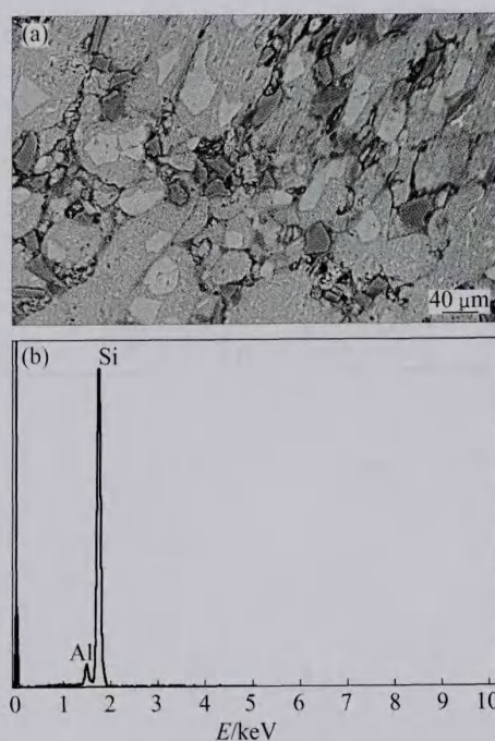
Fig. 7 SEM image (a) and EDS microanalysis (b) of selected point of Al–20SiC–12Si clad layer
