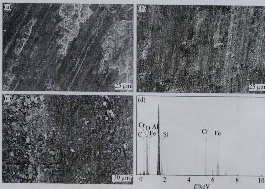
Fig. 10 SEM images of worn surfaces substrate (a), Al-20SiC (b) and Al-20SiC-7.2Si (c) clad layers and EDS analysis (d) of dark areas in Fig. 10(c)
