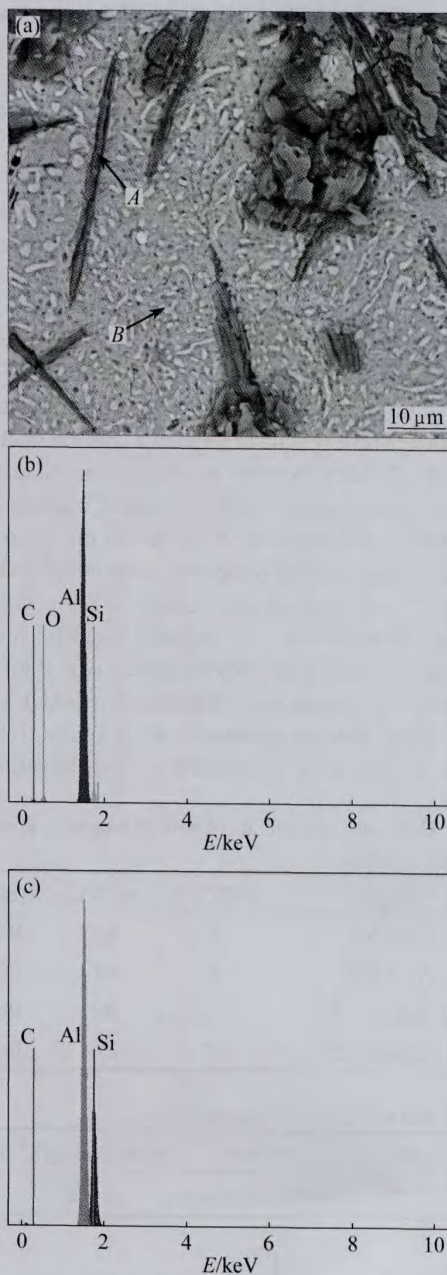
Fig. 4 Cross-sectional SEM image (a), EDS microanalysis of point A (b) and point B (c) of Al-30SiC clad layer
