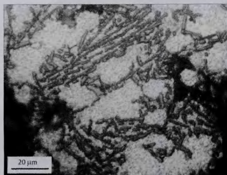
Fig. 6 Optical micrograph of Al–20SiC–7.2Si clad layer
