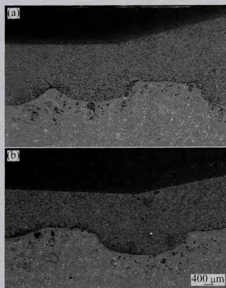
Fig. 5 Cross-sectional SEM images of Al–20SiC (a) and Al–30SiC (b) clad layers applied on aluminum alloy substrate
