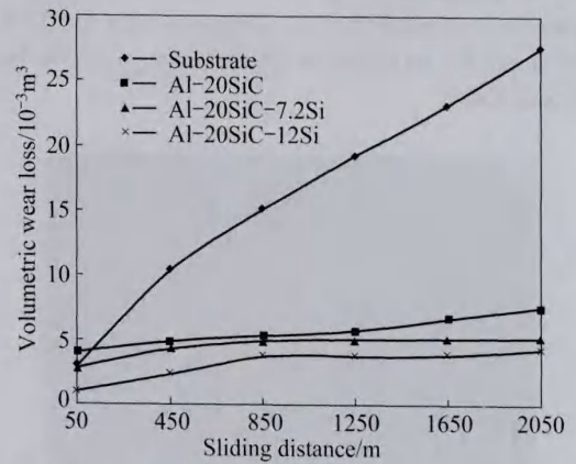
Fig. 9 Volume loss of different clad layers and substrate as function of sliding distance
