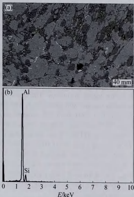
Fig. 2 Cross-sectional SEM image (a) and EDS microanalysis (b) of matrix of Al-20SiC clad layer
